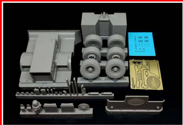
BRL32052 UK Flight Deck Tractor Tugmaster - resin/PE construction kit
